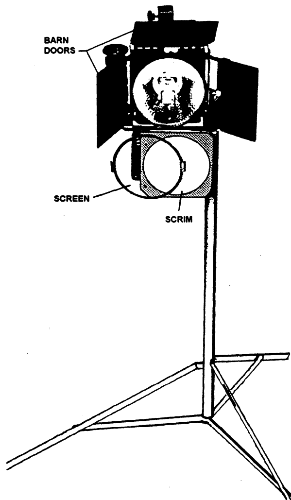
Figure 14-30.—Barn doors, screen and scrim.
