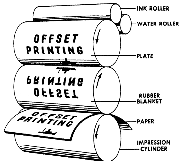
Figure 8-1.—The process of offset lithography.
