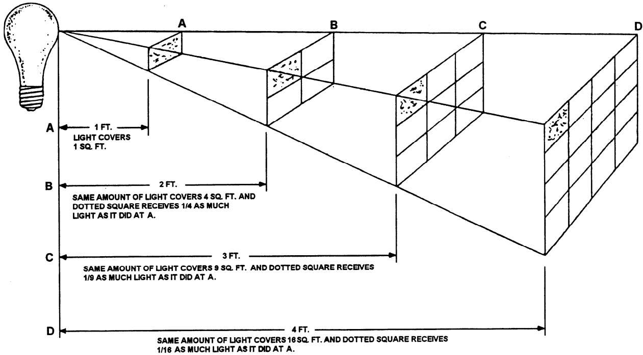
Figure 11-10.—Inverse-square law.
