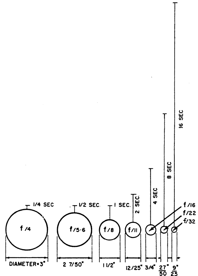
Figure 11-20.—Comparison between aperture, f/stop and relative exposure.
